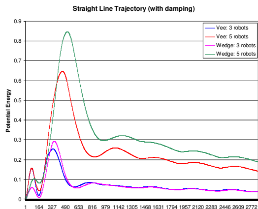
Fig. 11. Potential energy plots for the straight line trajectory.
