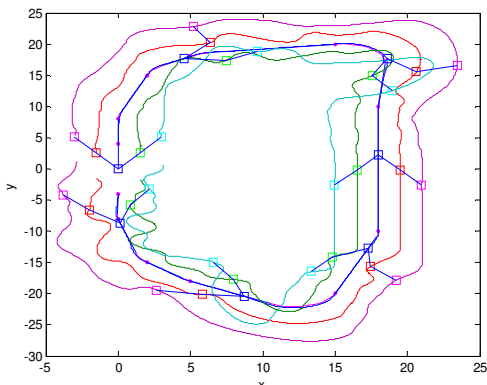
Fig. 10. Results obtained for the five robot system in the vee formation.
