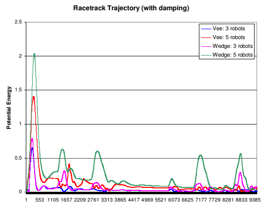
Fig. 12. Potential energy plots for the racetrack trajectory.
