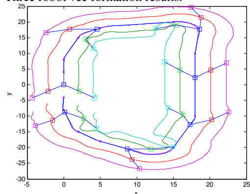
Fig. 9. Results obtained for the five robot system in the wedge formation.
