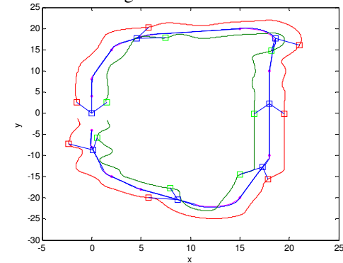
Fig. 8. Three robot vee formation results.
